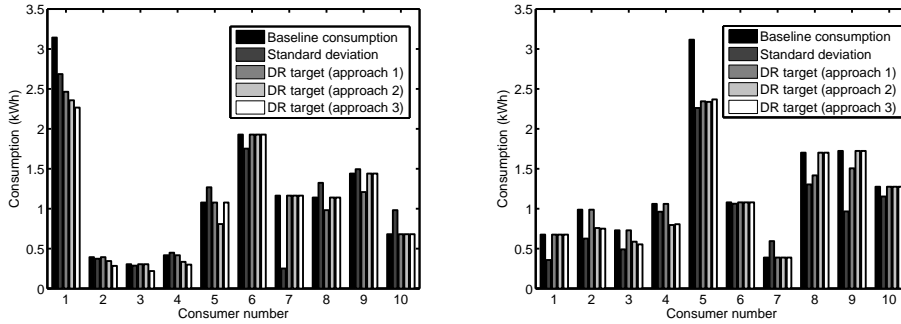
Figure 6: Comparison of DR target consumptions for consumers during time slots t = 13 (left) and t = 22 (right) using the first three optimization approaches. The baseline and standard deviation based on historical data are also shown for reference. Note that at t = 13 , while consumers with small baseline and standard deviation (e.g. 2 and 4) are never targeted in the deterministic case (approach 1), they can be targeted in the stochastic case (approach 2) due to their higher participation probabilities.
